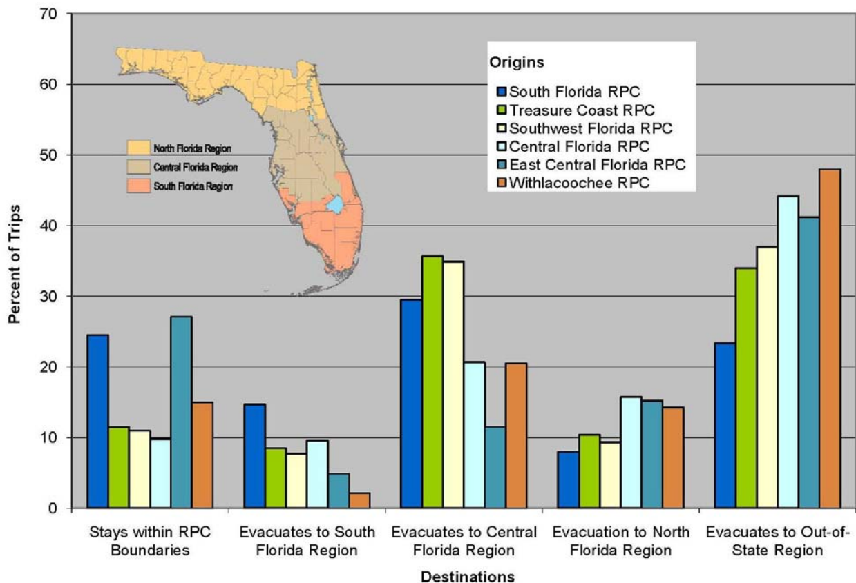
Figure 5.1.3: Average Evacuation Trip Distributions for Regional RPC Evacuations along the US 27 Corridor
